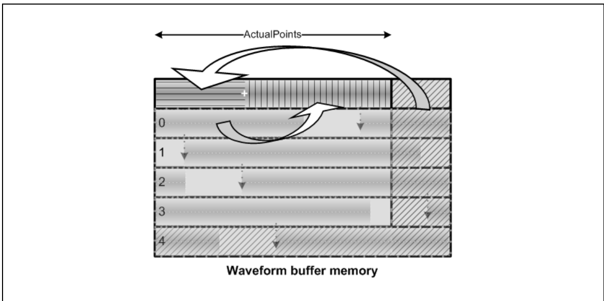
Figure 4-8 Reordering of the records
