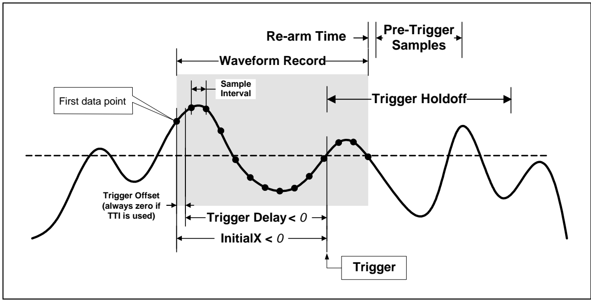
Figure 4-4 Negative Trigger Delay
