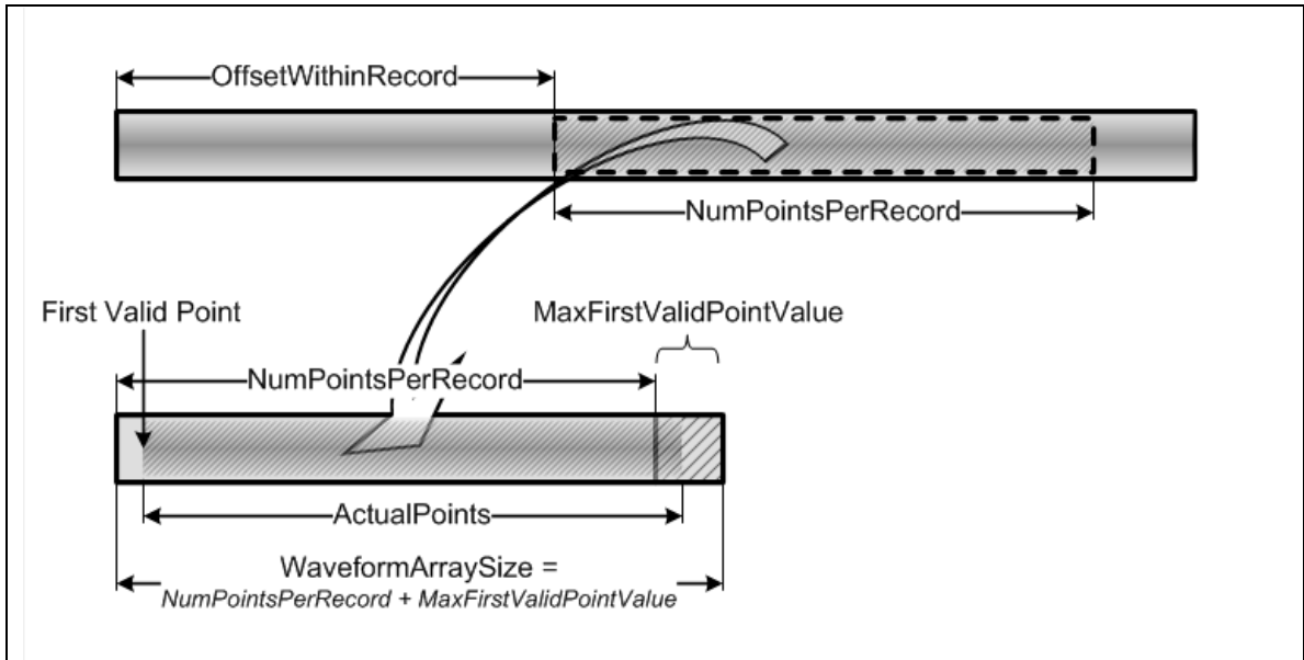
Figure 4-11 Retrieving a partial record
