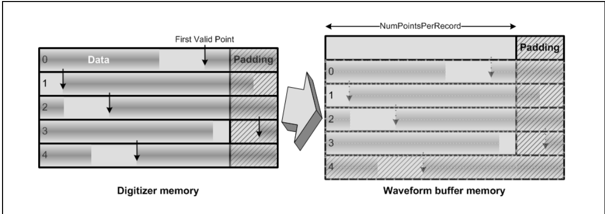
Figure 4-7 Multi-record transfer
